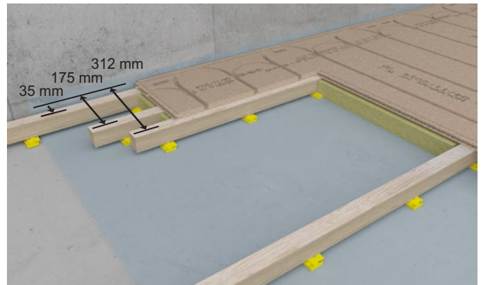
Figure 4 Climate Floor with edge joists 35 mm c-c from the wall and with extra joists under the turning grooves and under the joint between turning panels and floor boards, see installation instructions for Kronospan turning panels.
